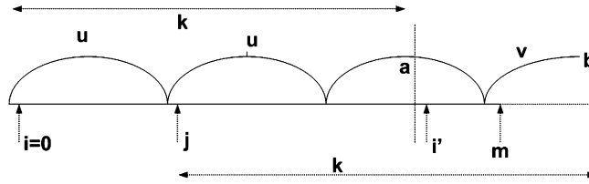
Fig. 2. The configuration when i is moved for the first time to some position i' : u^t v b is a prefix of w , \text{MaxSuf}(u^t v b) = v b , m = |v^t| , and the maximal suffix of the whole text does not start before m .
