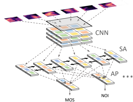
Figure 3: NISQA neural network architecture.
