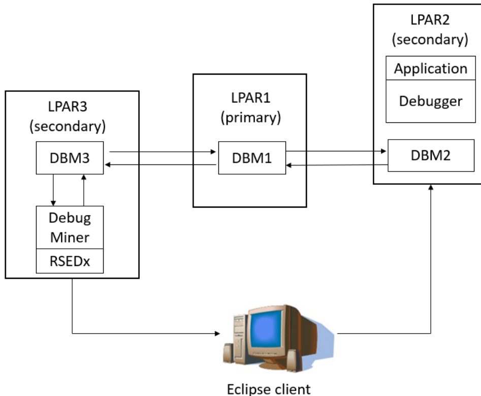
Figure 4. Debug Manager instances in a sysplex environment.
