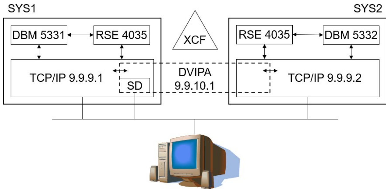
Figure 8. Distributed Dynamic VIPA sample
