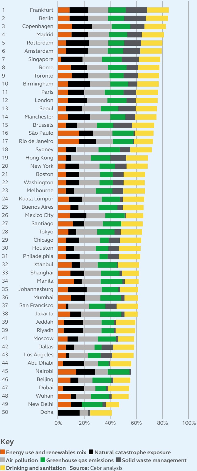
Figure 3: Two German cities score highest on environmental stability, with Europe performing strongly
