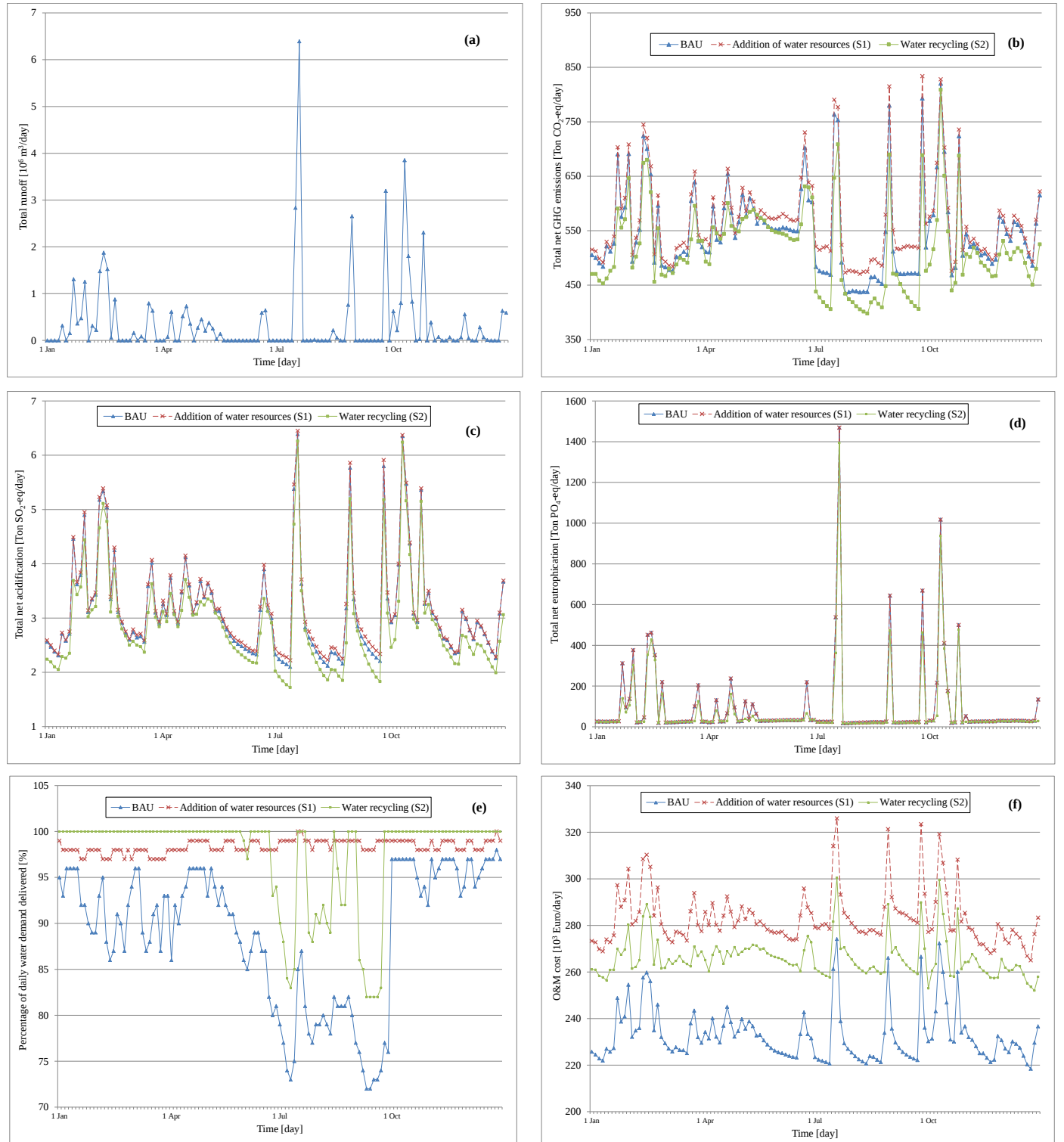
Fig. 10. Daily variations of the metrics for different strategies for (a) runoff (b) net GHG emissions (c) net acidification (d) net eutrophication, (e) water demand delivered, and (f) O&M cost.
