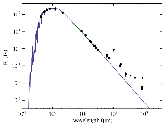
Figure 5. Observed SED of \tau Ceti. Circles are measured fluxes, while triangles show upper limits. Spitzer IRS data are shown in green, on top of the photospheric model (blue line). The observed data include fluxes obtained from optical (Bessel 1990; Perryman & ESA 1997; Hauck & Mermilliod 1998; Høg et al. 2000; Mermilliod 2006), 2MASS (Skrutskie et al. 2006), Spitzer (Chen et al. 2006), AKARI (Ishihara et al. 2010), IRAS (Moshir et al. 1990), ISO (Habing et al. 2001), JCMT (Greaves et al. 2004, Greaves et al. in preparation), and HHT (Holmes et al. 2003), as well as the Herschel PACS and SPIRE values and upper limits. See Tables 2 and 3 for values.
