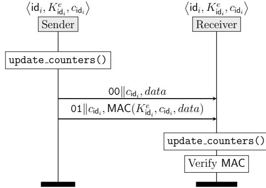
Figure 7. Message authentication between sender S and receiver R for message with identifier \text{id}_i , with command code.
