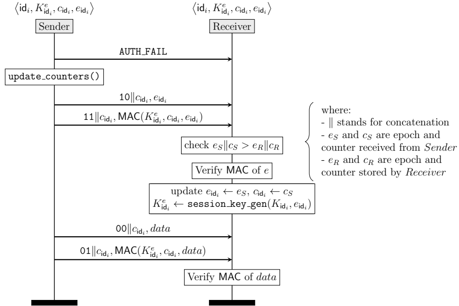
Figure 8. Message authentication failure and resynchronisation procedure, between sender S and receiver R for message with identifier \text{id}_i , with command code placement.
