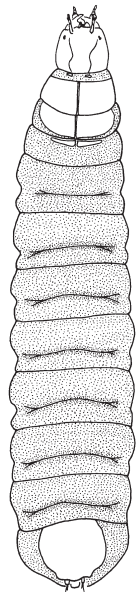
C. praetextatus larva (adapted from Archangelsky 1997)
