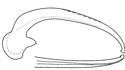
P. stagninus aedeagus, lateral view (above) and oblique dorsal view (below)
