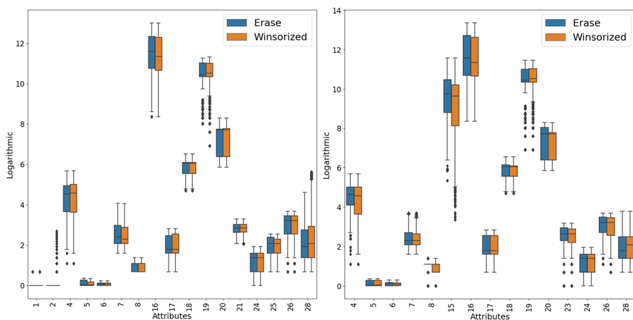
Fig. 5 Attributes with statistically significant differences (total number of minutes of delay). Variables are numbered as per Table 3
