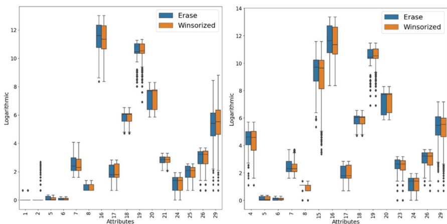
Fig. 6 Attributes with statistically significant differences (number of affected passengers). Variables are numbered as per Table 3
