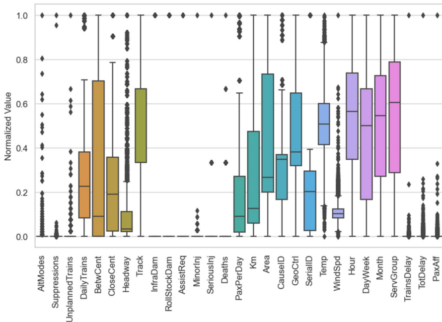
Fig. 3 Original dataset (normalized data)
