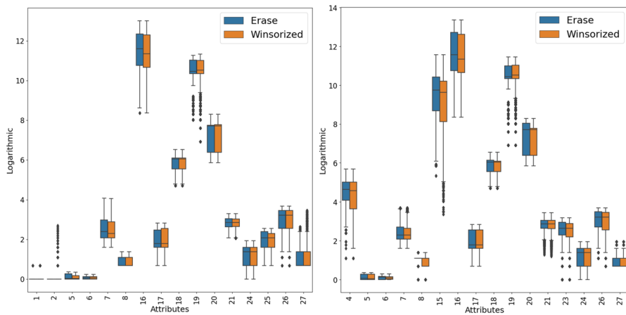
Fig. 4 Attributes with statistically significant differences (number of trains affected by delay). Variables are numbered as per Table 3
