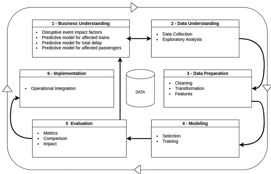
Fig. 1 The six phases of CRISP-DM, adapted from Martinez-Plumed et al. (2021)
