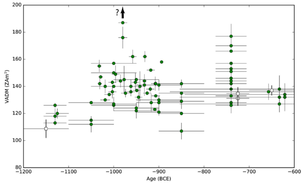
Figure 8: High resolution archaeointensity curve for the early Iron Age Levant indicating two ‘spikes’ of more than 170 ZAm 2 (after Shaar, et al., 2016). Data from the current study suggest that the earlier spike (around 980 BCE) might have reached intensity values of more than 200 ZAm 2 (cf., Ben-Yosef, et al., 2009) (see text). In turn, they also indicate Iron Age smelting at KHI and Giv’at Hazeva.
