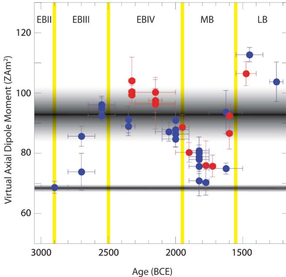
Figure 9: Results of the archaeomagnetic experiments of the current study plotted against geomagnetic values for the EB Age from Syria (Gallet, et al., 2014; in red data from Ebla and in blue from other sites). The EB II-III and EB III-IV boundaries are after the new absolute dating of Regev et al. (2012a, 2012b). The geomagnetic values from the EB Age copper production sites of the southern Levant fall into two tight groups, of high intensities (around 90 VADM ZAm^2 ), and low intensity (around 68 VADM ZAm^2 ). The shading represents standard deviation of the general mean; cf. Table 2.
