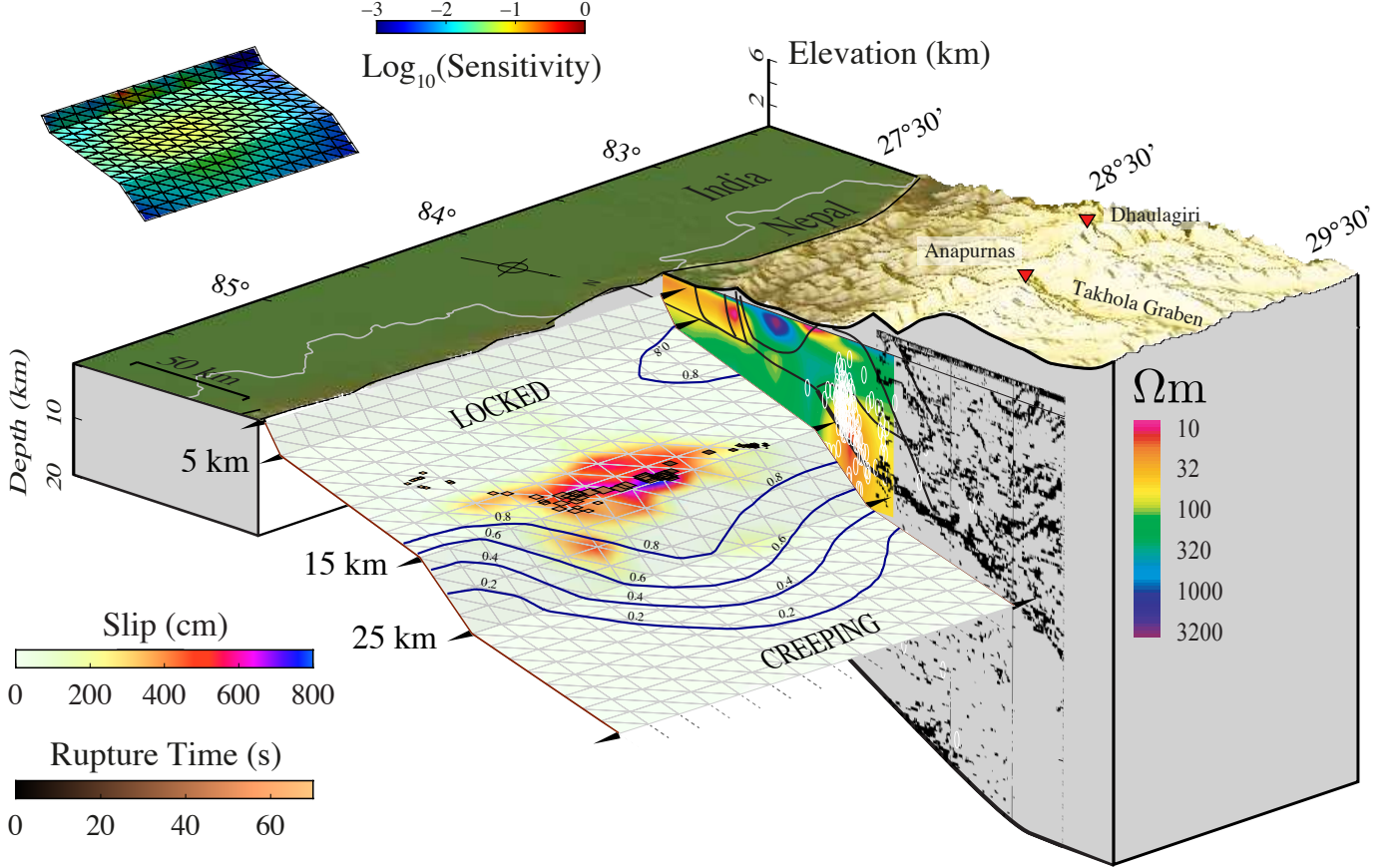
Figure 4 | Three-dimensional block diagram of the geometry proposed for the MHT. Colors denote earthquake slip relative to interseismic coupling (blue lines) inferred from GPS-, leveling- and InSAR-derived deformation rates prior to the Gorkha earthquake 25 . High-frequency seismic sources 1 during the earthquake rupture (diamonds), run along the ramp-and-flat hinge line at 14–15 km depth. The cross-section shows the InDepth reflection profile 15 , the main faults (black lines) and an electromagneto-telluric image 23 highlighting the high-conductivity measured along the MHT. White ellipses are relocated micro-seismic activity prior to the Gorkha earthquake. Note the gap between the fault plane and cross section for clarity. Inset: Model sensitivity S (defined as diag(\mathbf{G}'\mathbf{G}) where \mathbf{G} is the Green's function matrix) indicates the normalized sum of surface displacements caused by unit slip on each point on the fault.
