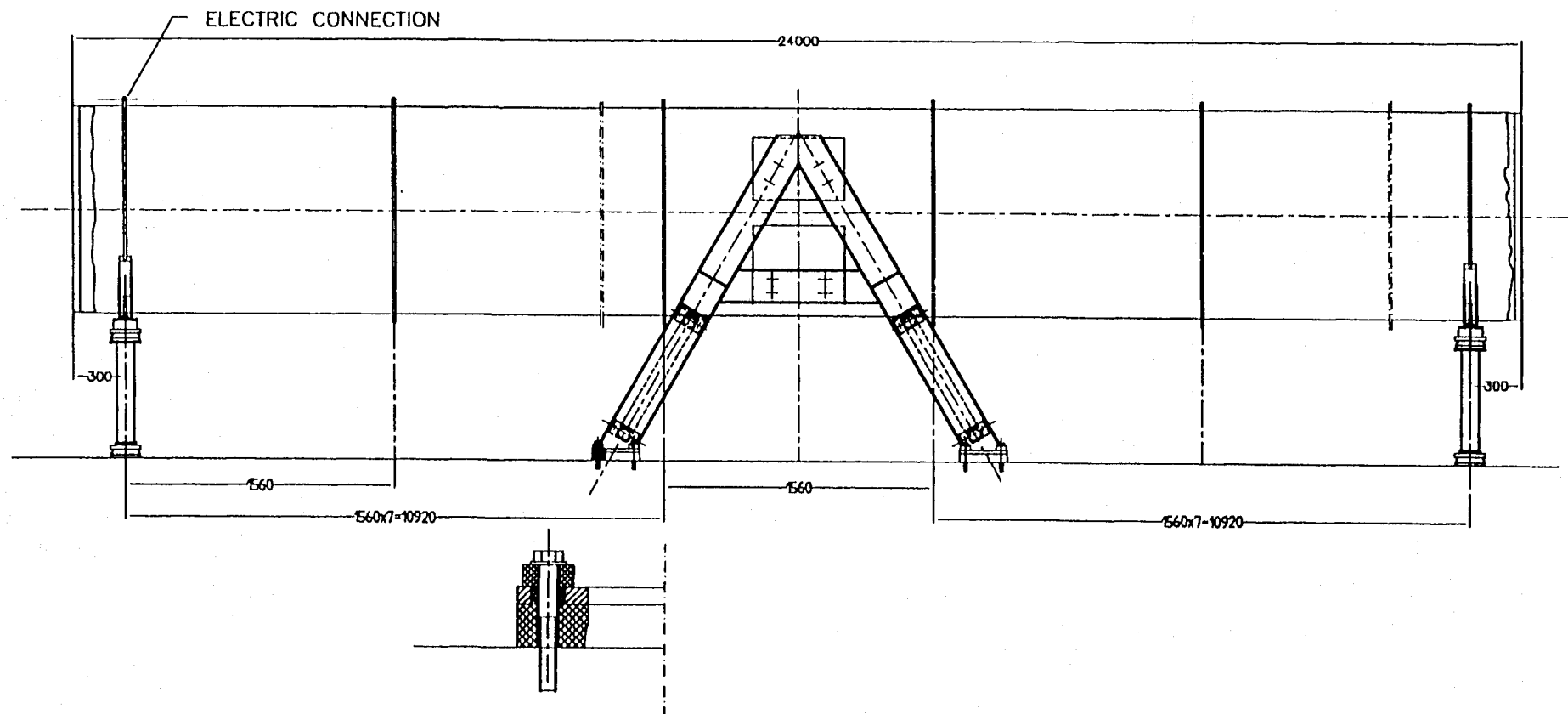
Fig.5 INITIAL MODULE (VTIM1001)
