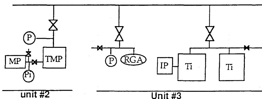
Synopsis of the intermediate and permanent pumping of the tube (unit #2 and 3)
