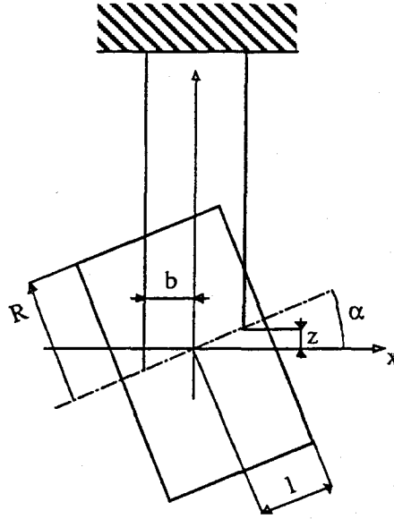
Figure 5: Tilt mode of a suspended cylindrical mirror
