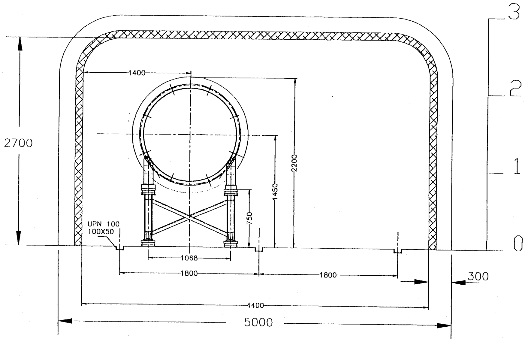
Fig.6 CROSS SECTION OF TUNNEL
