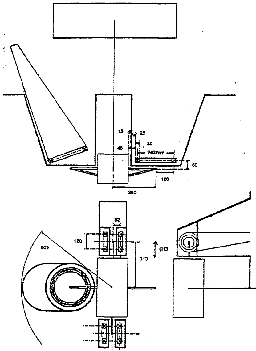
Figure 3: The last stages of the suspension.
