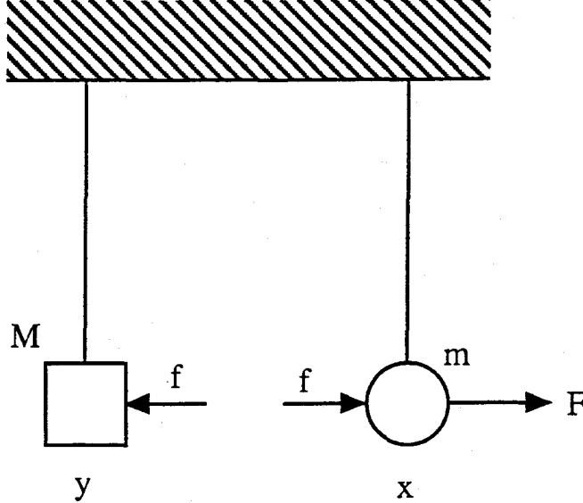
Figure 6: Model of coupled mirror-reference mass system.
