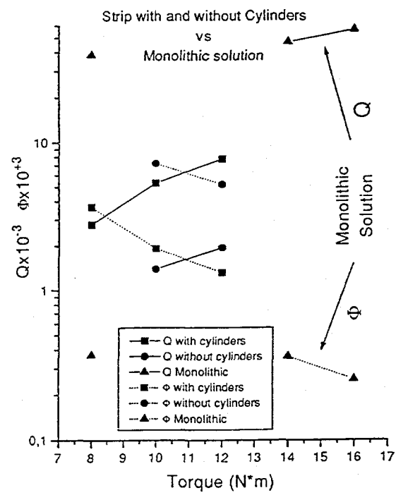
Figure 10: Future developments: Monolithic prototype
