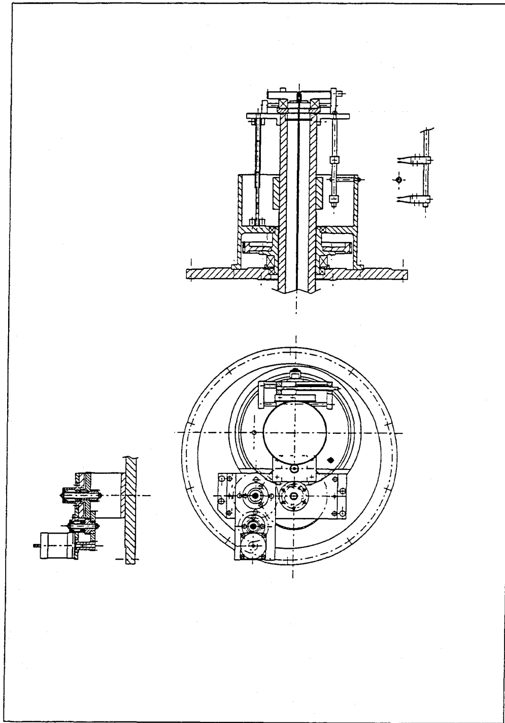
Figure 7: The micrometric table lift.
