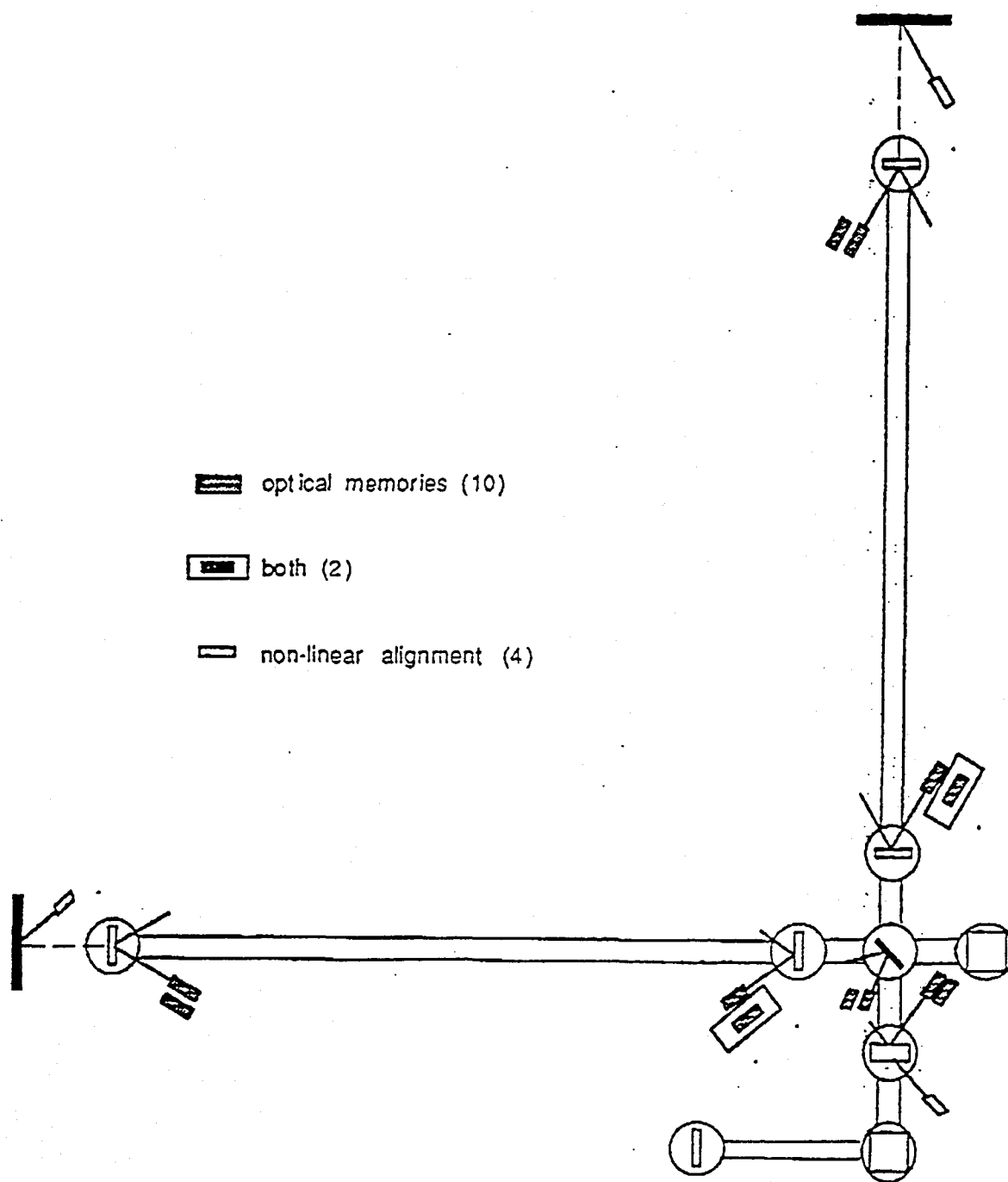
Fig. 3: layout of the 16 CCD cameras.
