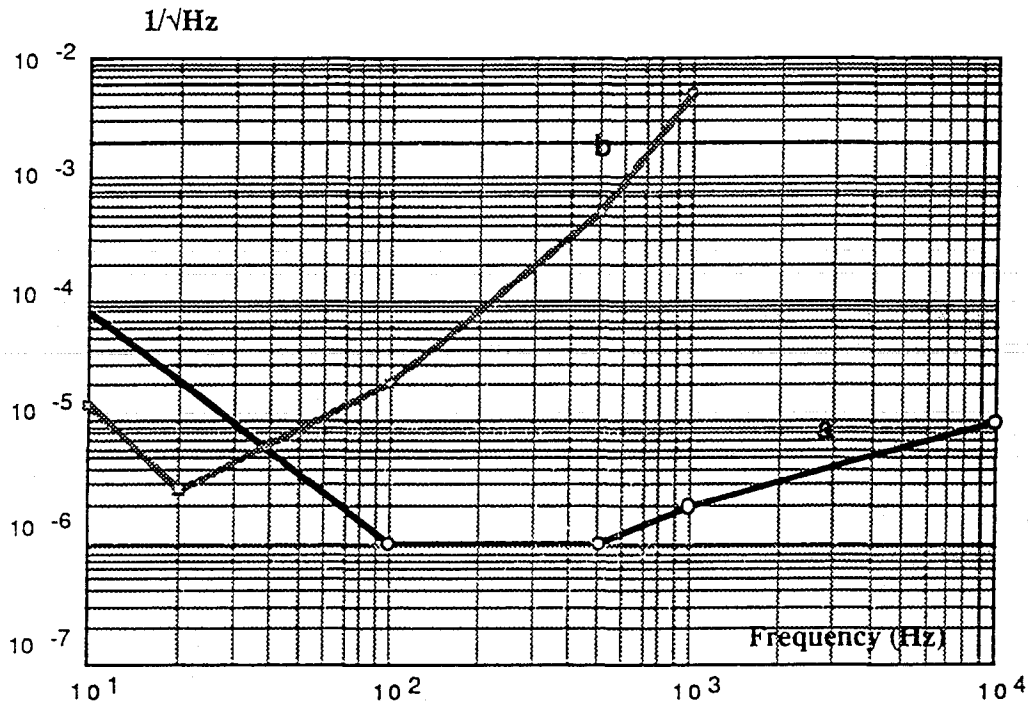
Figure III.5.1.a : Requirement on relative amplitude stability, curve a : due to residual error in mass position, curve b : due to radiation pressure on test-mass.
