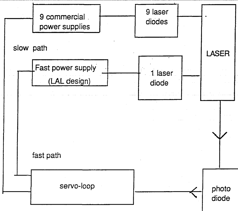
Figure III.5.3.a : Block Diagram of the laser intensity stabilization : the feed back is performed on one of the 10 laser diodes using to optically pump the high power laser.
