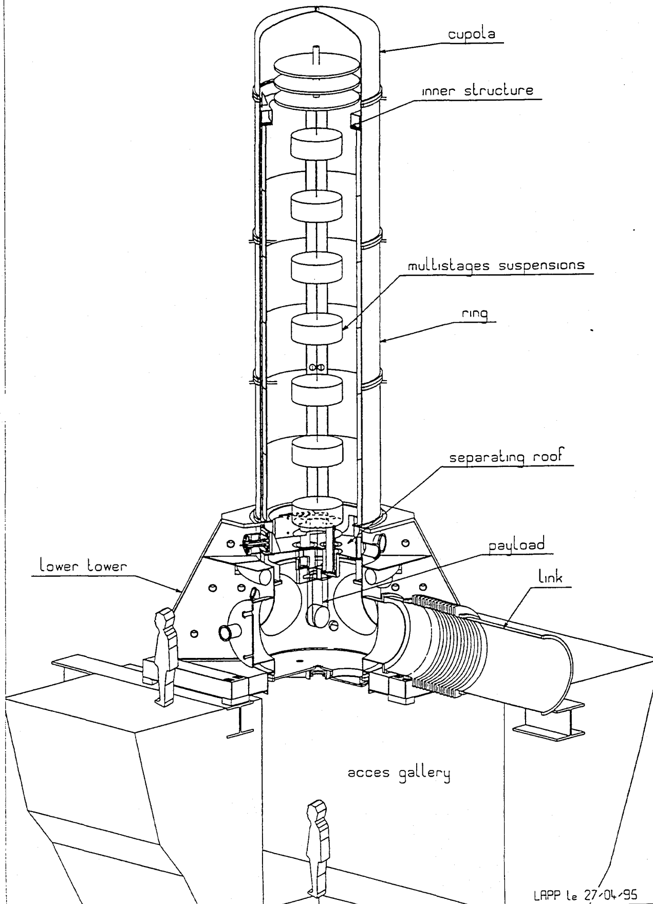
TOWER MAIN COMPONENTS
