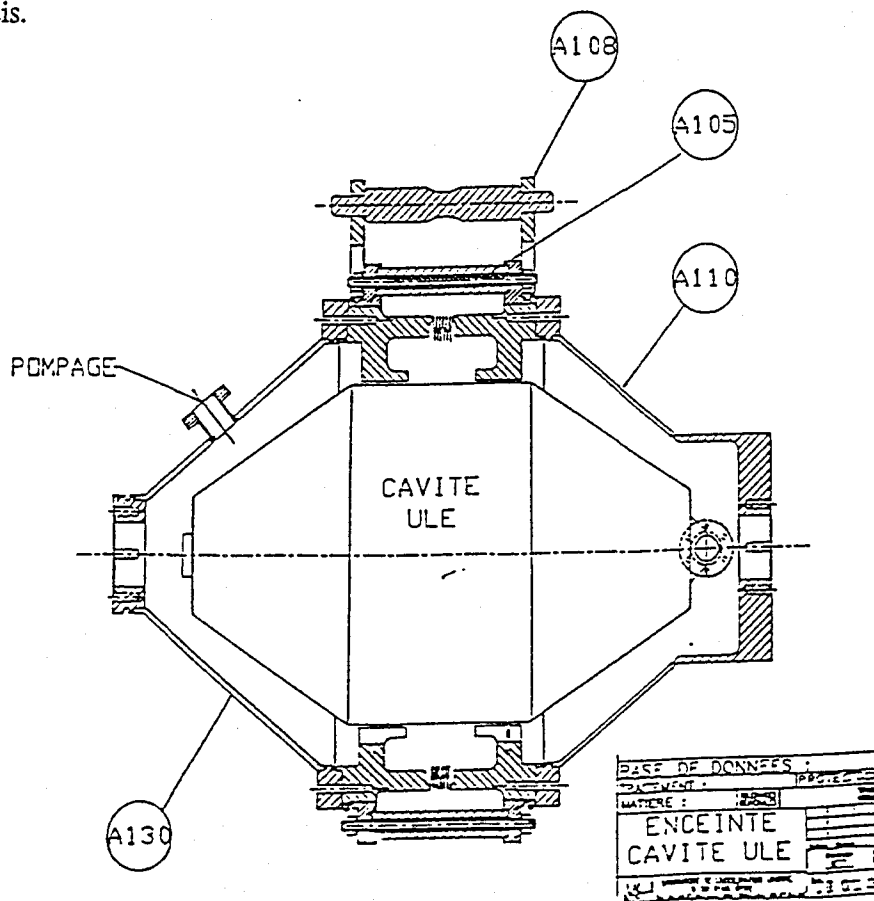
Figure II.3.3.b: Reference Cavity and its vacuum housing
