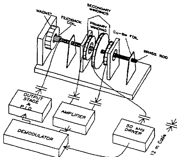
Figure 1: Linear accelerometer structure.
