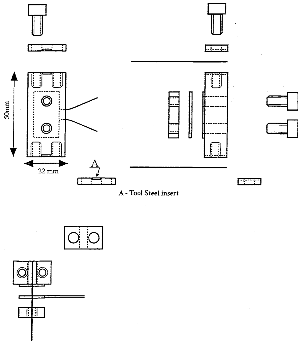
Figure 11: Suspension wire clamp design
