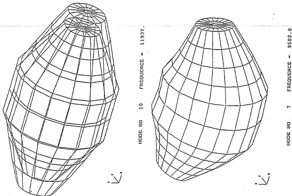
Figure II.3.3.a: Reference Cavity shape and first mechanical resonances calculated by a finite element analysis.
