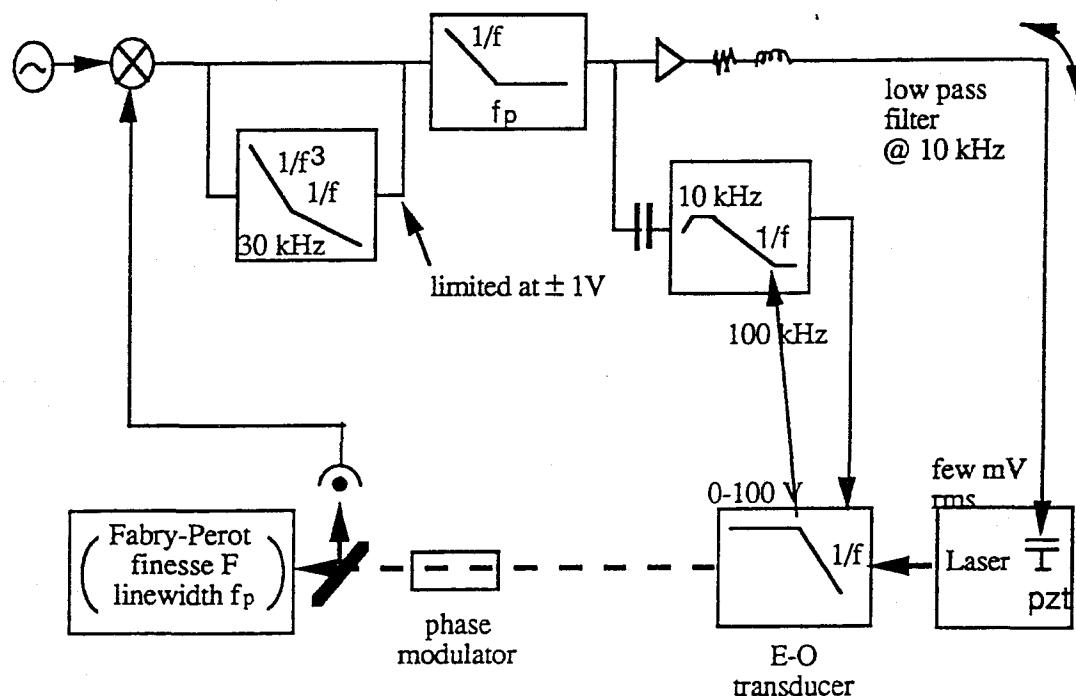
Figure IL3.4.a : Servo-loop diagram of the prestabilization
