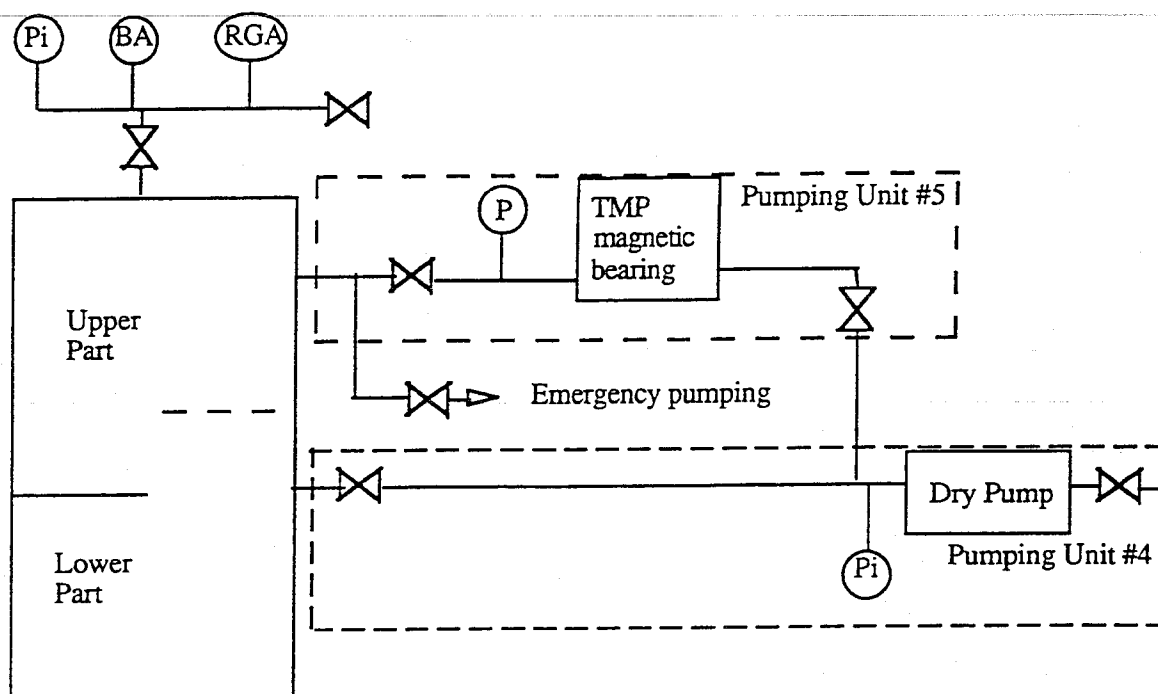
Synopsis of the pumping of a mirror tower (unit #4 and 5)
