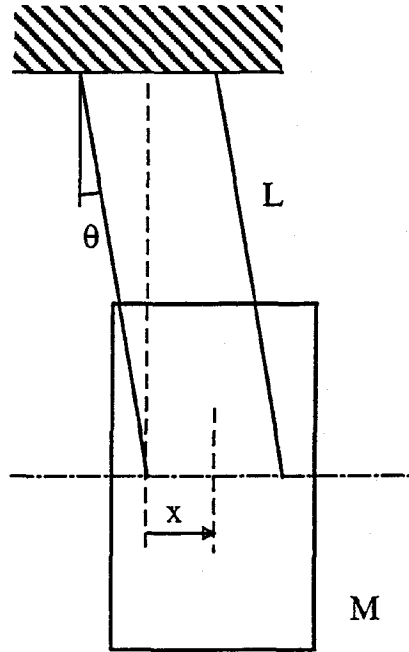
Figure 1: Simple pendulum
