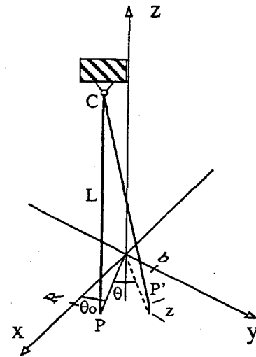
Figure 4: Rotational mode coordinates of a suspended cylindrical mirror
