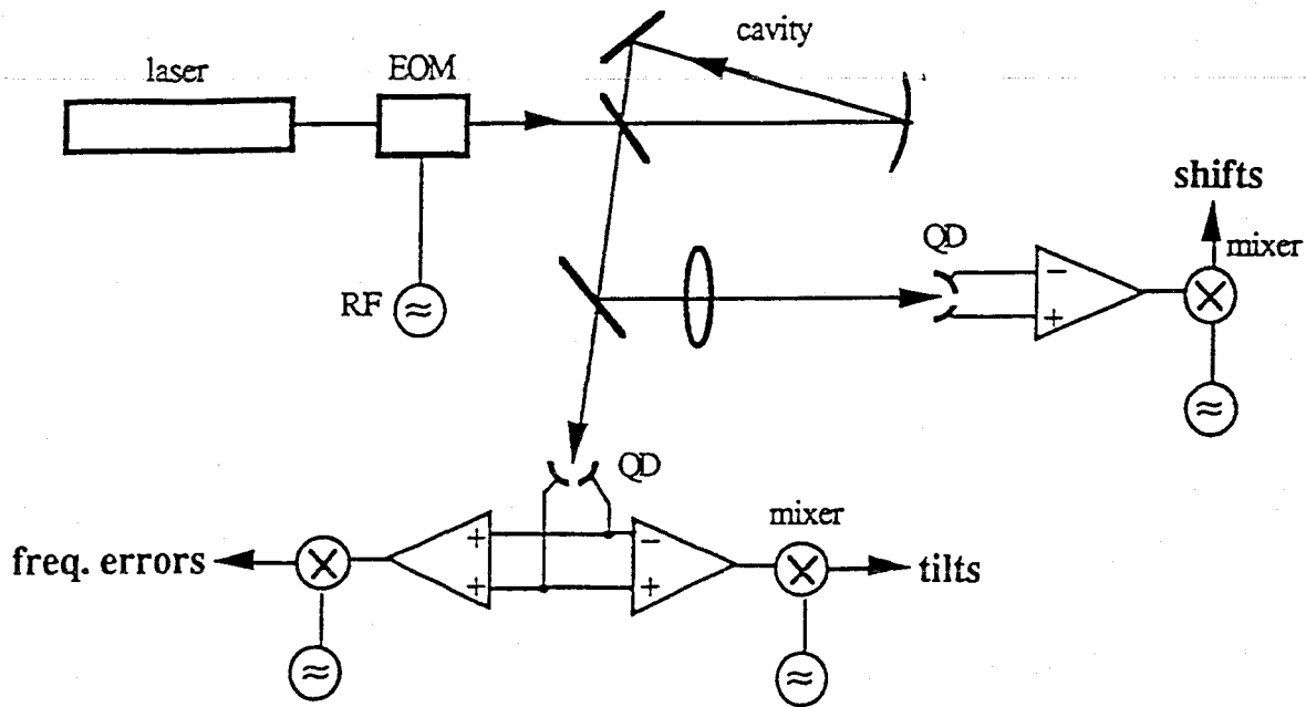
Figure IV.6.1.a : Typical setup for measuring the alignment (and frequency) errors of a laser with respect to a cavity. (EOM=electro-optical modulator; QD=quadrant photodiode; RF=radio frequency generator).
