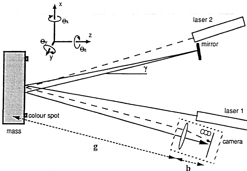
Figure IV.4.1.a: Optical scheme for determining the mass position with a camera, similar to the one proposed by Annecy. The spot generated by laser 1 serves for determining \theta_x , \theta_y ; the image of the two points on the CCD gives x, y and \theta_z ; laser 2 gives informations on z .
