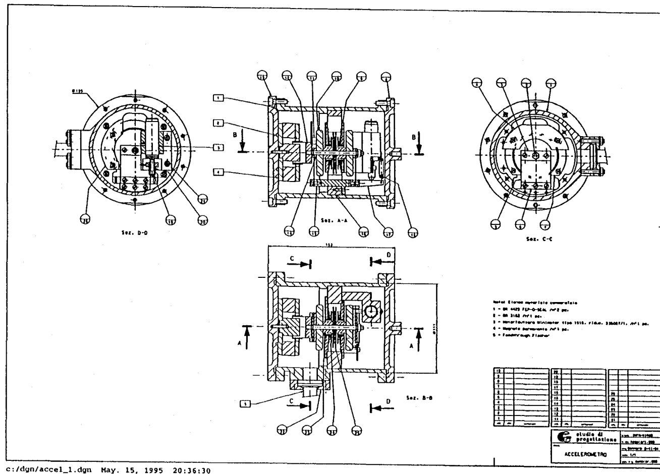
Figure 3: The linear accelerometer.
