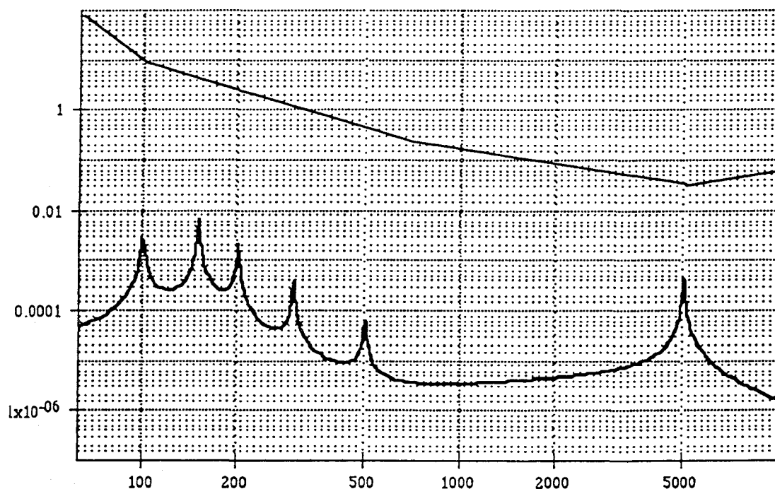
Figure III.3.3.a : Equivalent frequency fluctuation induced by corner-cube MC thermal noise of mass M=1 kg, Q=100 , resonance at 5kHz and by the IB (4 resonances between 100 and 400 Hz). The upper curve is the Virgo requirement on the laser noise after the MC.
