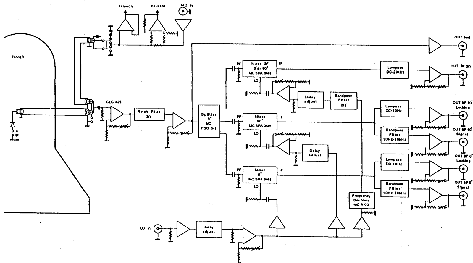
Fig VII-3. Schematic implantation of a detection channel
