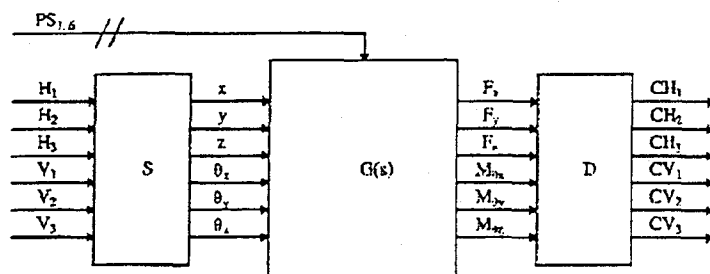
Figure 2: Damping system feedback.
