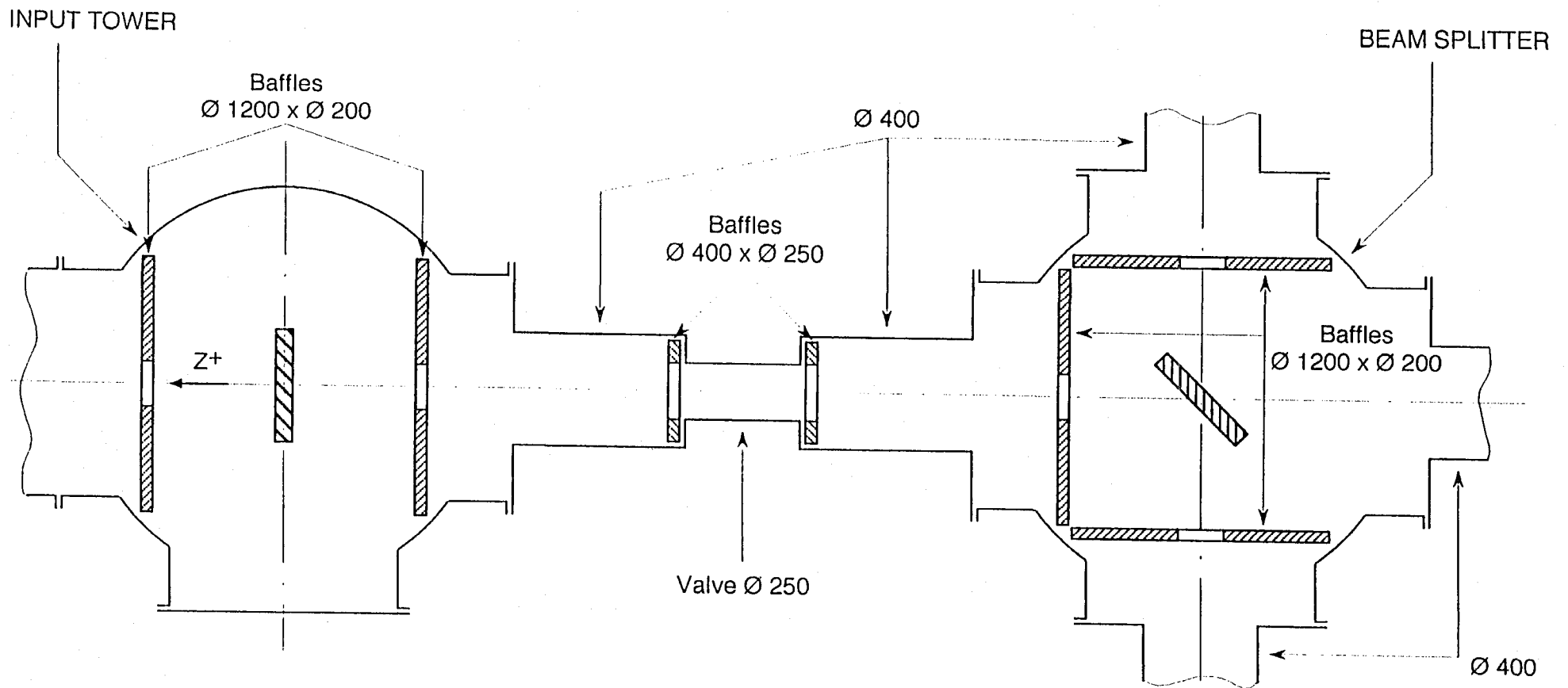
Fig. 4 Baffles in the central area
