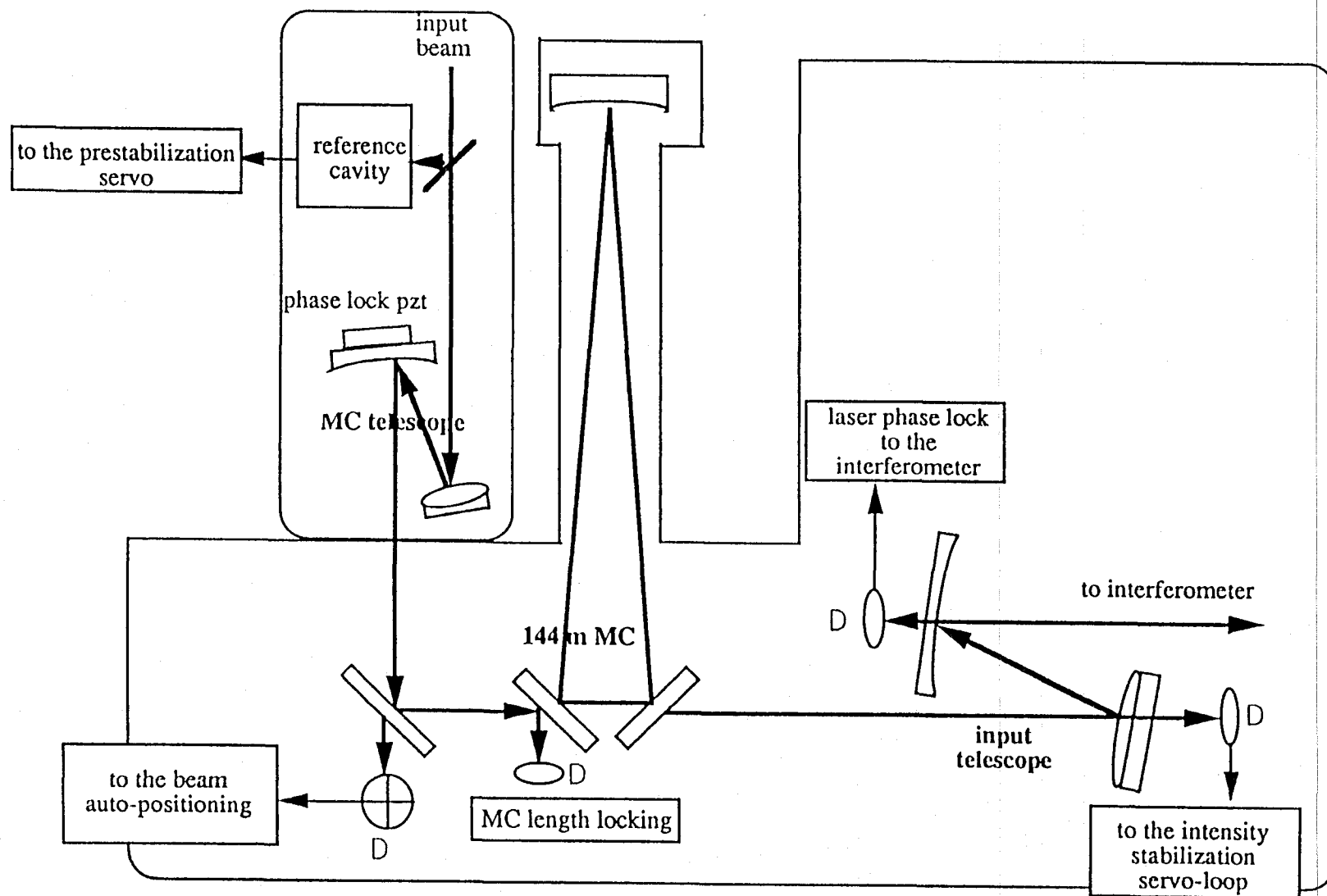
Figure III.1.a : Schematic of the Input Bench
