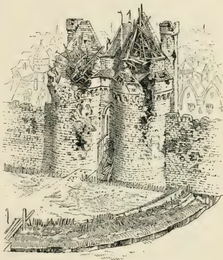
FIG. 198. EFFECTS OF CANNON ON A MEDIEVAL CASTLE
