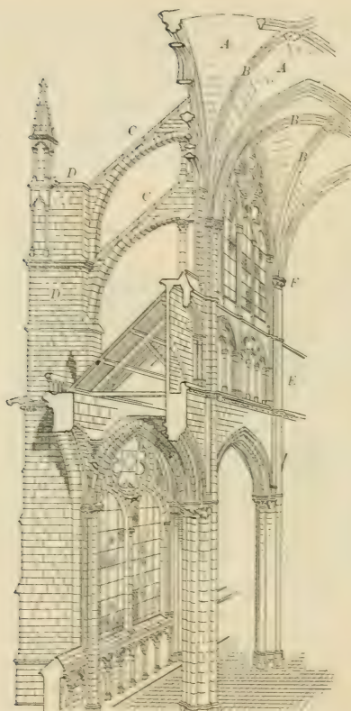
FIG. 183. CROSS SECTION OF AMIENS CATHEDRAL
