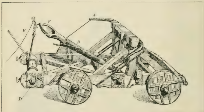
FIG. 153. MACHINE FOR HURLING STONES
