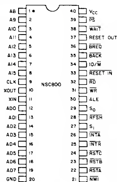
Figure 1. NSC800 pin configuration.
