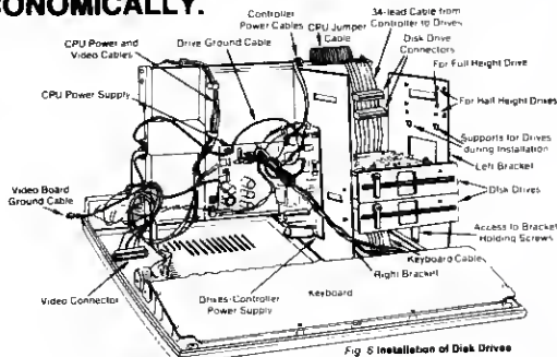
Fig. 5 Installation of Disk Drives
